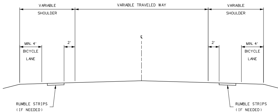
BICYCLE LANE ON SHOULDER
