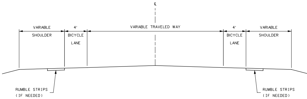
BICYCLE LANE ADJACENT TO TRAVELED WAY
