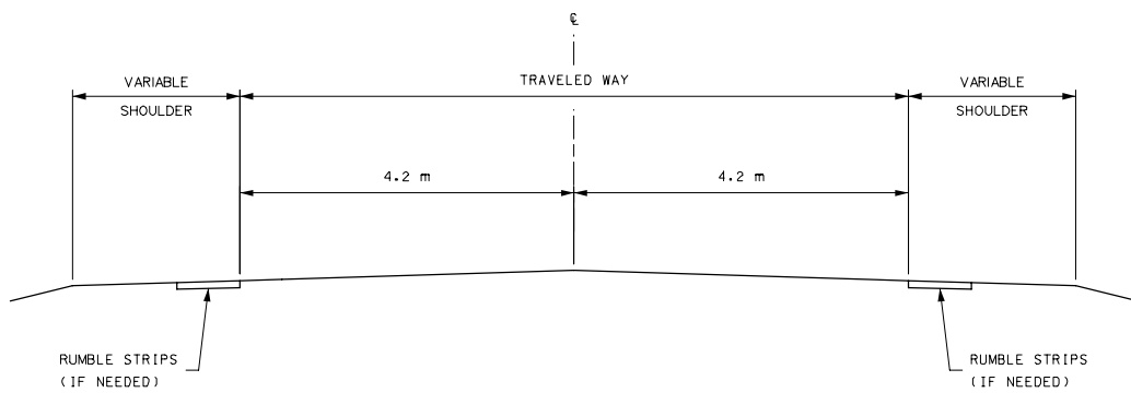
WIDE SHARED LANE
